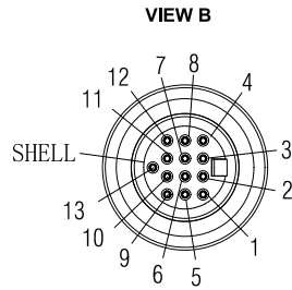
13 PIN FEMALE MATING FACE
